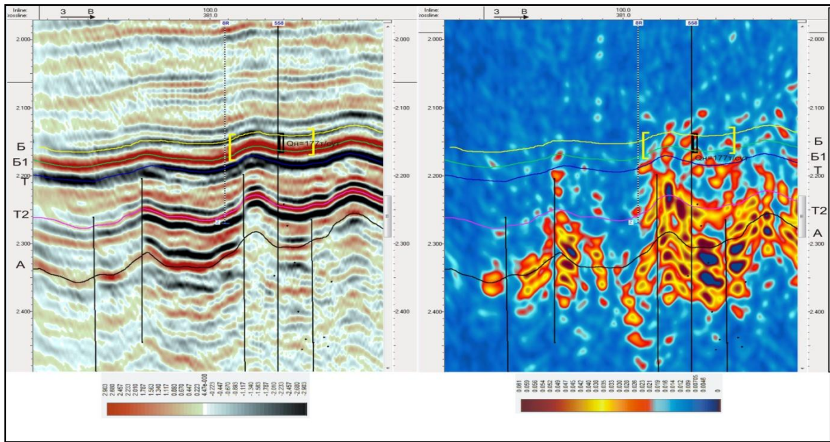
Figure 3 Reflectors (left) and diffractors (right) time sections
