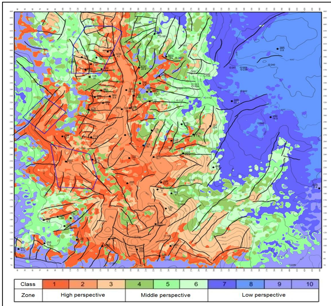
Figure 4 Perspective oil reservoirs map of Bazhen formation based on cluster analysis
